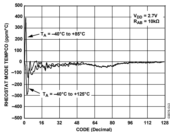
Figure 15. \Delta R_{WB}/\Delta T vs. Code
